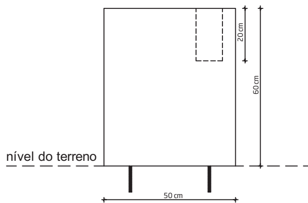
VISTA FRONTAL
